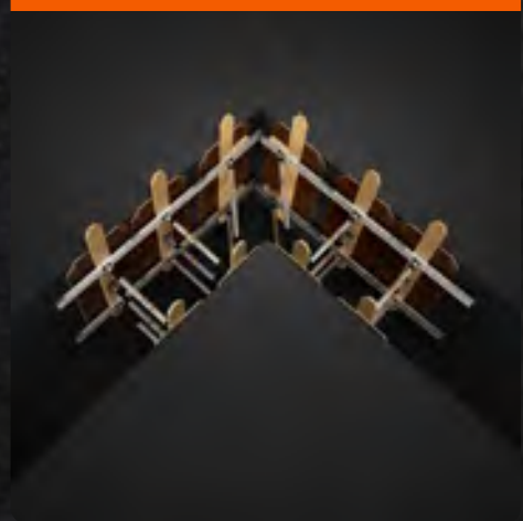
Trench shoring
